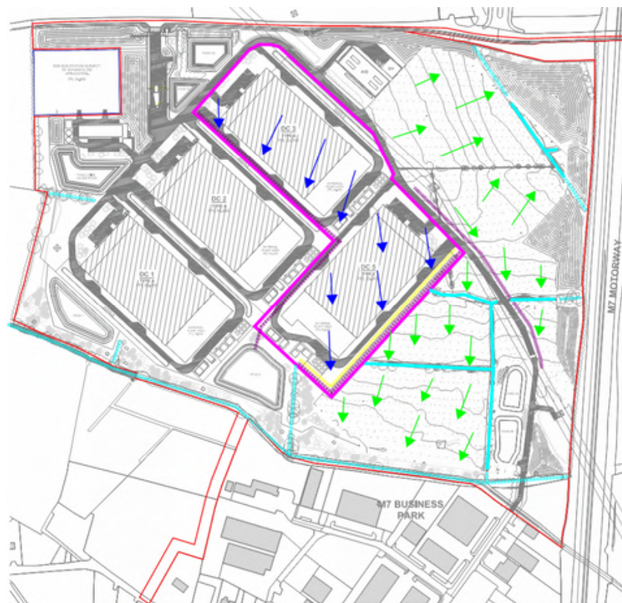
Figure 6-7 Phase 2 Overland Flow Strategy
